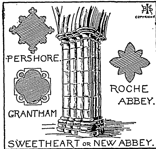
FIG. 45.—PIER TYPES.
